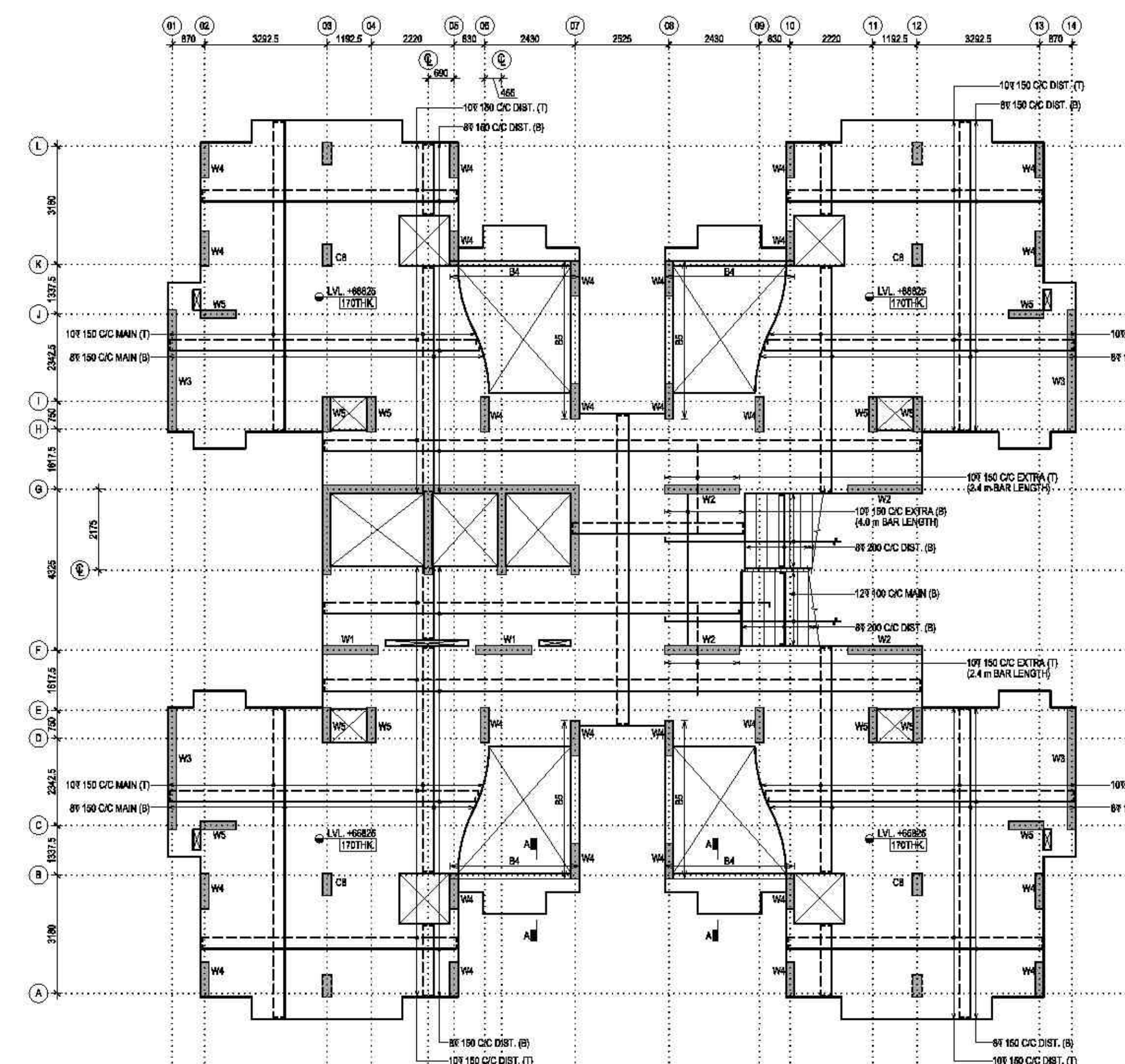
PENT HOUSE FLOOR LEVEL PLAN (+66825 LVL.)
